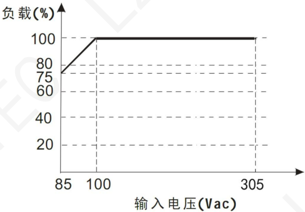
INPUT VOLTAGE VERSUS LOAD DIAGRAM
